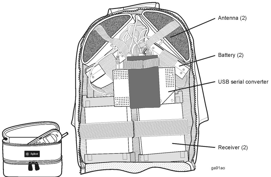
Figure 1-1 Arranging receivers and phones
