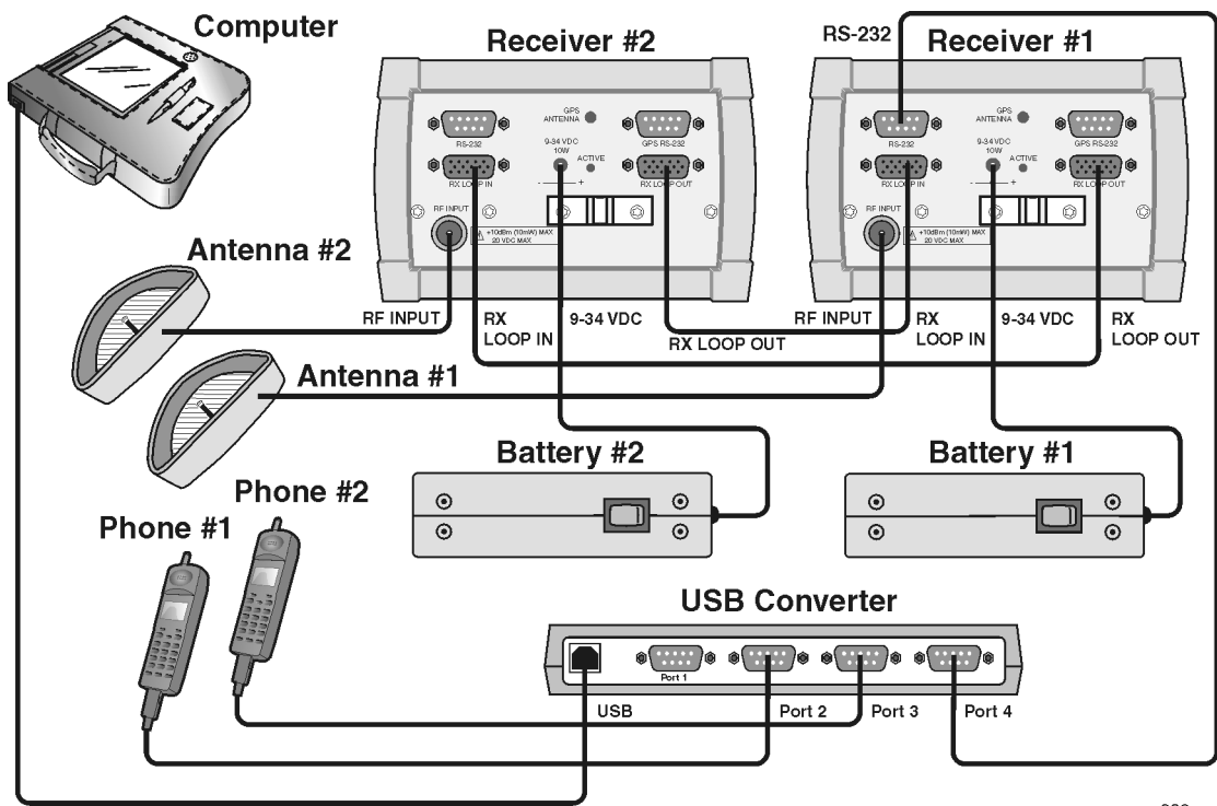
Figure 1-6 Connecting receivers and phones via the USB serial converter
